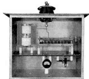
D-99418 (5 KW Shunt Type) Antenna Coupling Unit. (With cover removed.)
